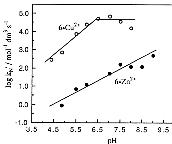
Fig. 11. pH-Rate profiles for the acylation rate constant k_N' for the metal ion complex of ligand 6 in HTAB micelles, 25^\circ\text{C} .
